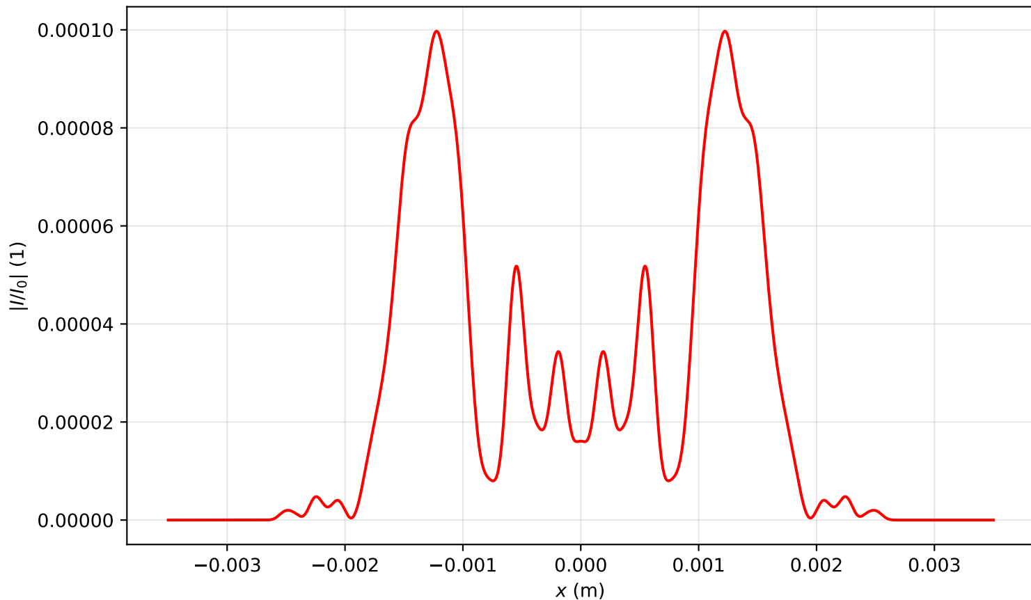
Intensity profile I(x, y = 0, z = 2.548)/I_0 , P_{in}=9.0P_{cr} , artificial time
